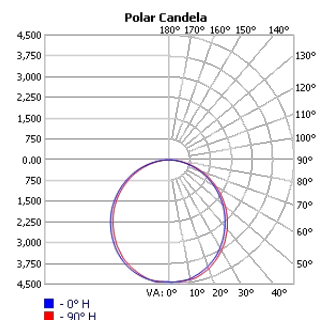
TECHOLED-ASH-D-35-HI-30
