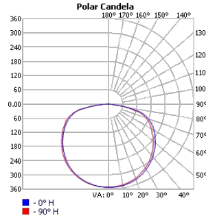
TECHOLED-ASR-D-14-ME-30
