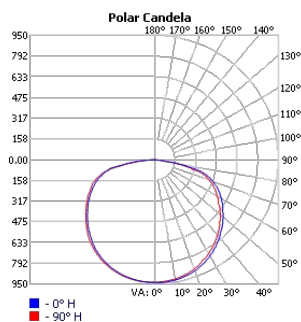
TECHOLED-ASR-D-31-LO-30
