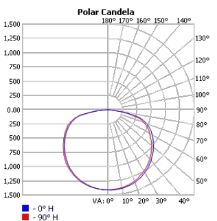
TECHOLED-ASR-D-31-HI-30
