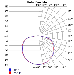
TECHOLED-ASR-D-14-HI-30
