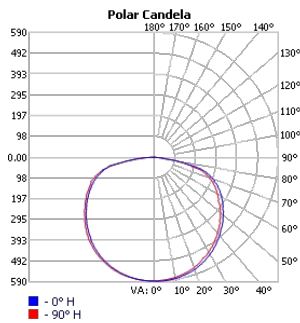
TECHOLED-ASR-D-17-ME-30
