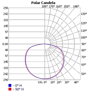
TECHOLED-ASR-D-14-LO-30
