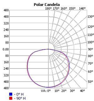
TECHOLED-ASR-D-17-LO-30
