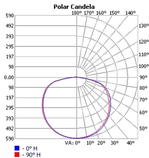
TECHOLED-ASR-D-23-LO-30
