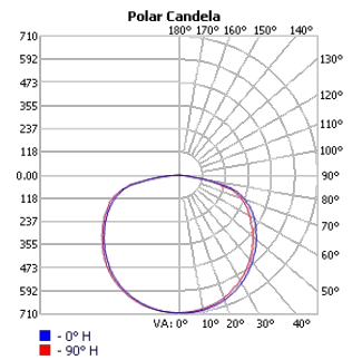
TECHOLED-ASR-D-17-HI-30
