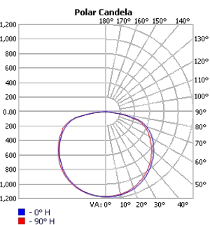
TECHOLED-ASR-D-31-ME-30
