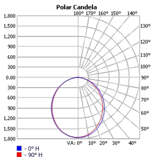
TECHOLED-BX-2P-D-8-LO-30
