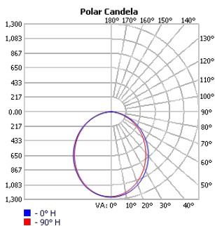
TECHOLED-BX-2P-D-6-LO-30
