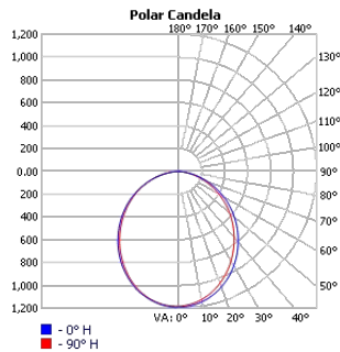
TECHOLED-BX-2P-D-4-ME-30
