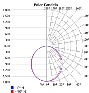
TECHOLED-BX-2P-D-6-ME-30
