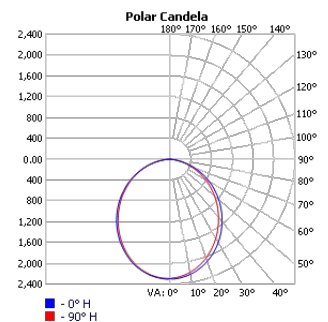
TECHOLED-BX-2P-D-6-HI-30
