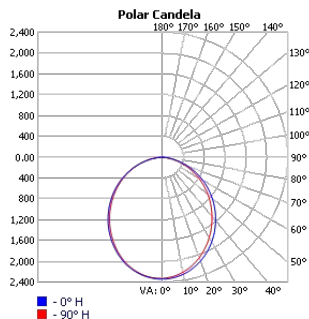
TECHOLED-BX-2P-D-8-ME-30
