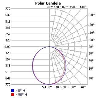
TECHOLED-BX-2P-D-2-HI-30
