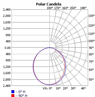
TECHOLED-BX-2P-D-8-ME-30
