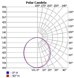
TECHOLED-BX-2P-D-4-LO-30
