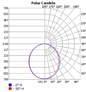
TECHOLED-BX-2P-D-2-ME-30
