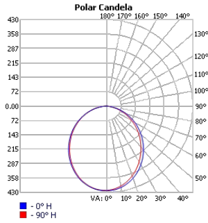
TECHOLED-BX-2P-D-2-LO-30
