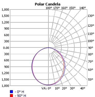
TECHOLED-BX-2P-D-8-LO-30
