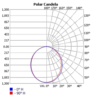
TECHOLED-BX-2P-D-6-LO-30
