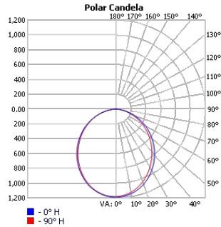
TECHOLED-BX-2P-D-4-ME-30
