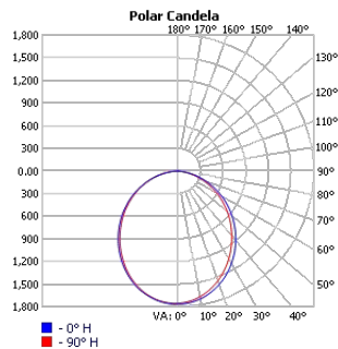
TECHOLED-BX-2P-D-6-ME-30
