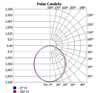
TECHOLED-BX-2P-D-8-HI-30
