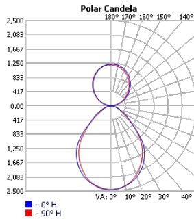
TECHOLED-BX-3RG-DI-6-ME-30
