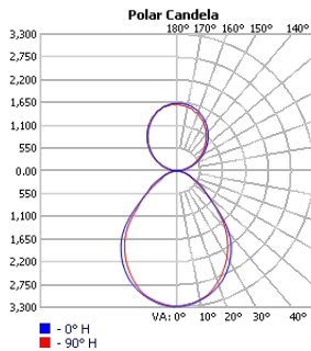
TECHOLED-BX-3RG-DI-8-ME-30
