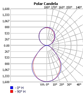
TECHOLED-BX-3RG-DI-6-LO-30
