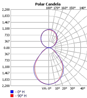
TECHOLED-BX-3RG-DI-8-LO-30
