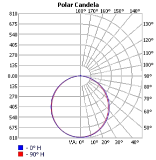
TECHOLED-BX-4-R-D-2-HI-30
