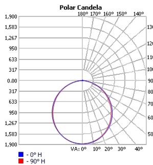
TECHOLED-BX-4-R-D-6-ME-30
