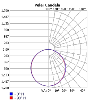
TECHOLED-BX-4-R-D-8-LO-30
