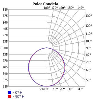
TECHOLED-BX-4-R-D-4-LO-30
