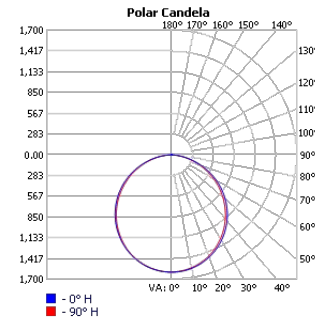
TECHOLED-BX-4-R-D-4-HI-30
