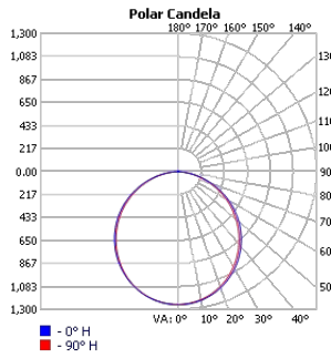
TECHOLED-BX-4-R-D-4-ME-30
