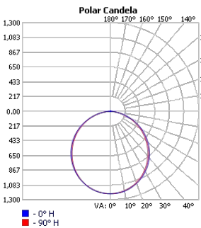
TECHOLED-BX-4-R-D-6-LO-30
