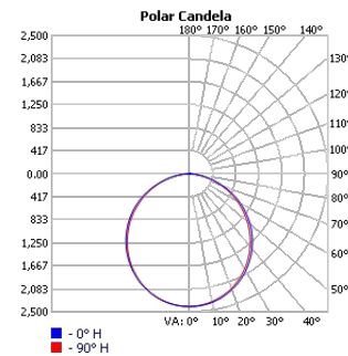
TECHOLED-BX-4-R-D-6-HI-30
