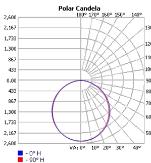
TECHOLED-BX-4-R-D-8-ME-30
