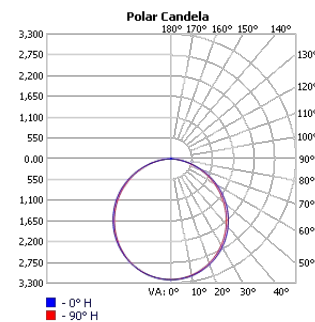
TECHOLED-BX-4-R-D-8-HI-30
