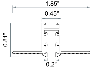
Recessed (RP)
