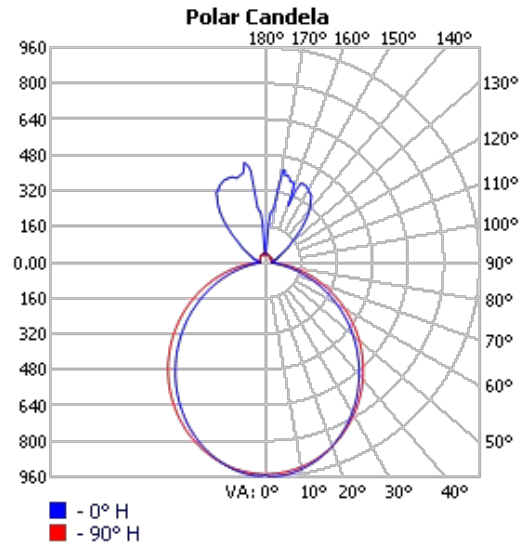
Direct/Indirect
